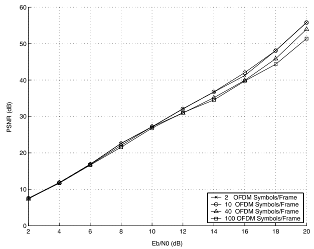
Fig. 11. PSNR performance for different frame sizes.
