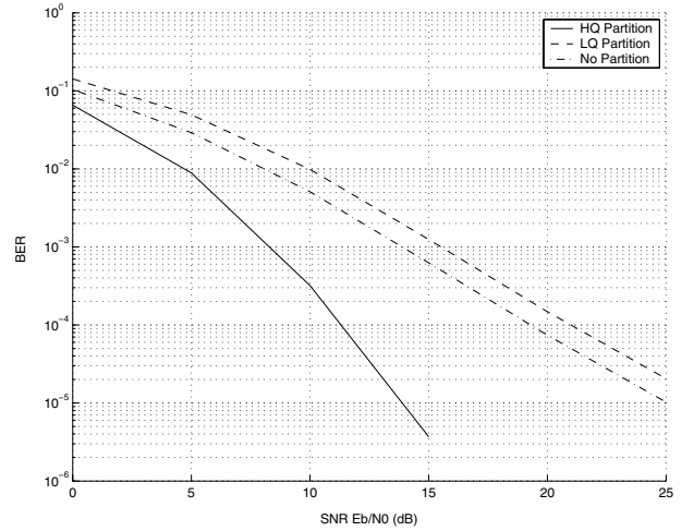
Fig. 7. Performance of different sub-channel partitions.
