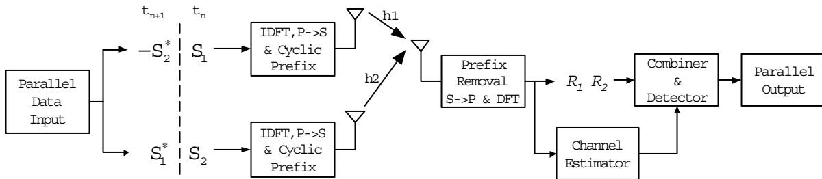
Fig. 2. An STBC-OFDM system.
