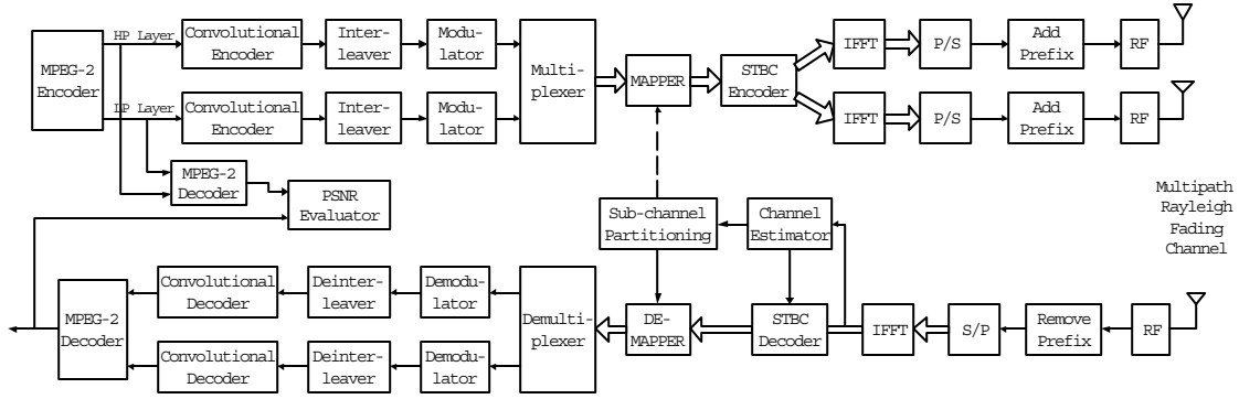
Fig. 5. System schematic.
