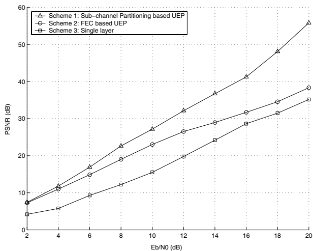
Fig. 8. PSNR performance of different schemes.
