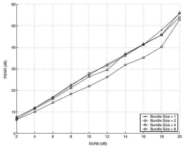
Fig. 12. PSNR performance for different sub-channel bundle sizes.
