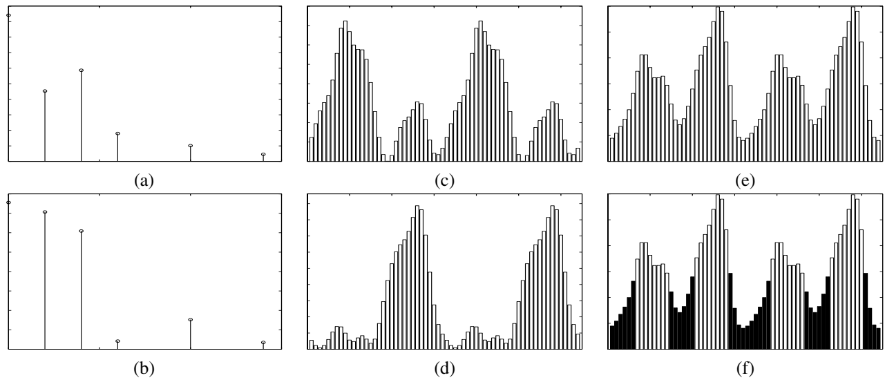
Fig. 3. An example of sub-channel partitioning. (a) time domain representation of multipath channel 1 (from transmit antenna 1 to the receive antenna): \mathbf{h}_1 ; (b) time domain representation of multipath channel 2 (from transmit antenna 2 to the receive antenna): \mathbf{h}_2 ; (c) squared frequency domain response of channel 1: |\text{DFT}(\mathbf{h}_1)|^2 ; (d) squared frequency domain response of channel 2: |\text{DFT}(\mathbf{h}_2)|^2 ; (e) composite channel response: |\text{DFT}(\mathbf{h}_1)|^2 + |\text{DFT}(\mathbf{h}_2)|^2 ; (f) sub-channel partitioning based on composite channel response.
