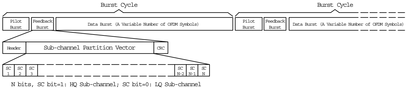
Fig. 4. Burst Structure.
