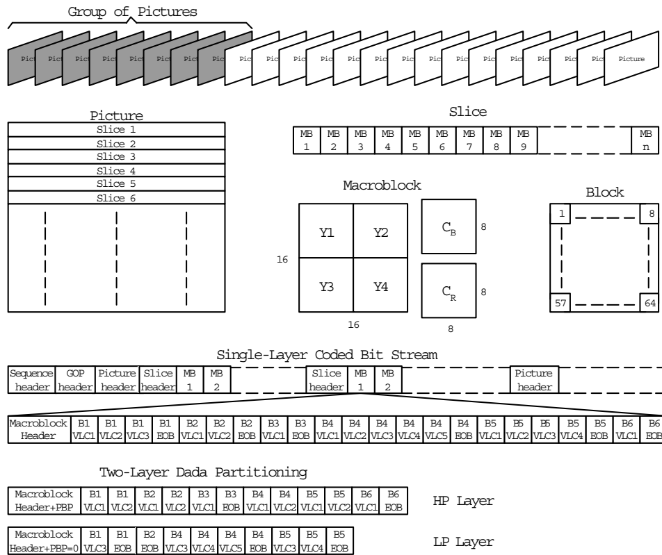
Fig. 1. Structure of MPEG data and data partitioning.
